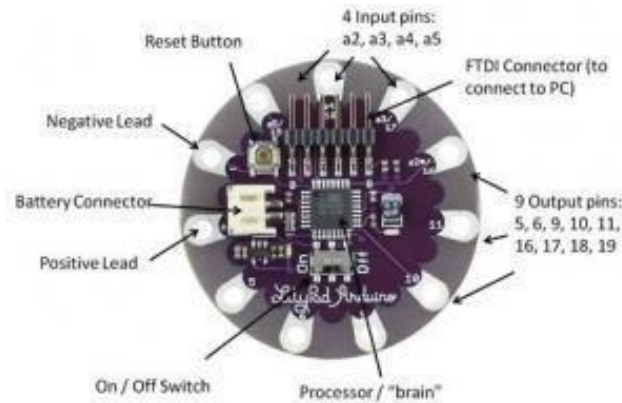
LilyPadArduinoBoards
