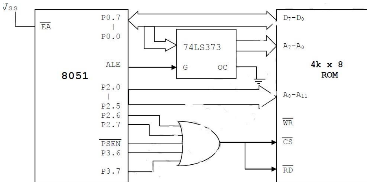
Figure 4Kx8 Memory (ROM) Interfacing with 8051
